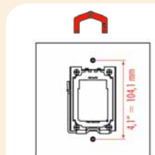
Socket G34 / Socket F
