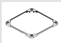
8x NA-AVP1-LR load-relief anti-vibration pads
